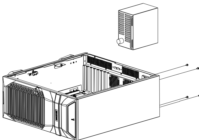
Figure 3.6: Replacing the power supply/ 更换电源 / 更換電源
