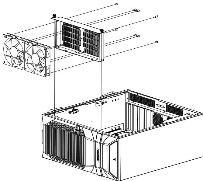
Figure 3.4: Replacing system fan/ 更换系统风扇 / 更換系統風扇
