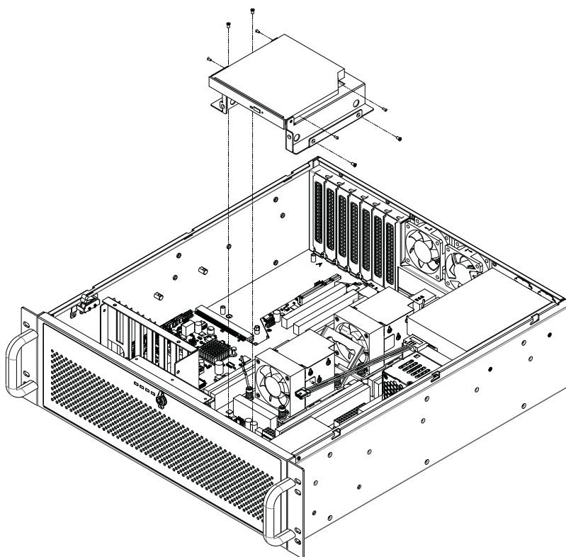
Figure 2.5 Installing the slim-type optical disk drive/ 安装薄型光驱 / 安裝薄型光碟機
