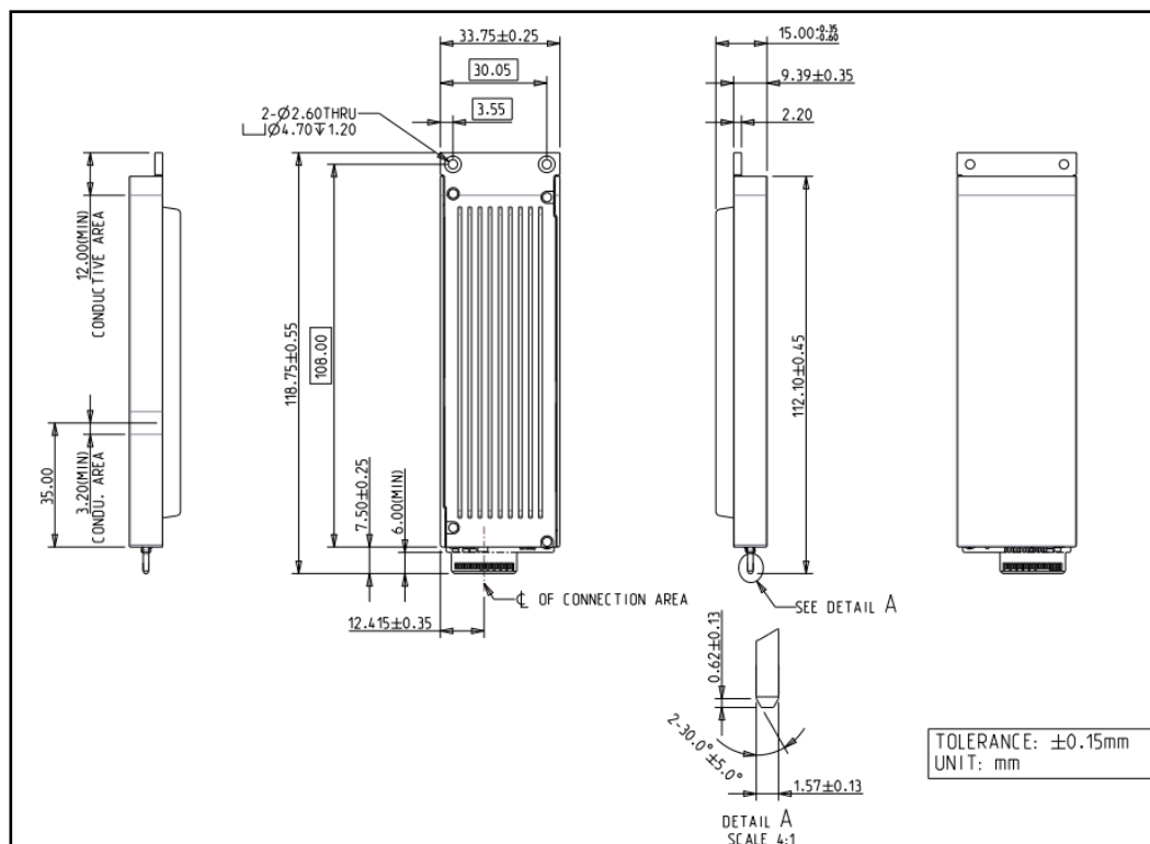
EDSFF 1U short with 15mm asymmetric heat-spreading enclosure
