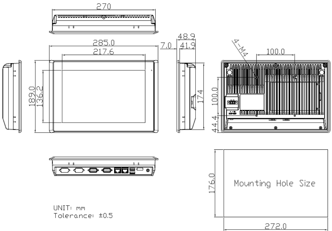
Figure 1.3: Dimensions of ARCHMI-710(P)
