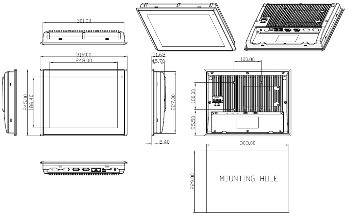
Figure 1.4: Dimensions of ARCHMI-712(P)
