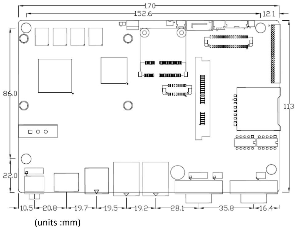
Figure 2.1: Mainboard Dimensions
