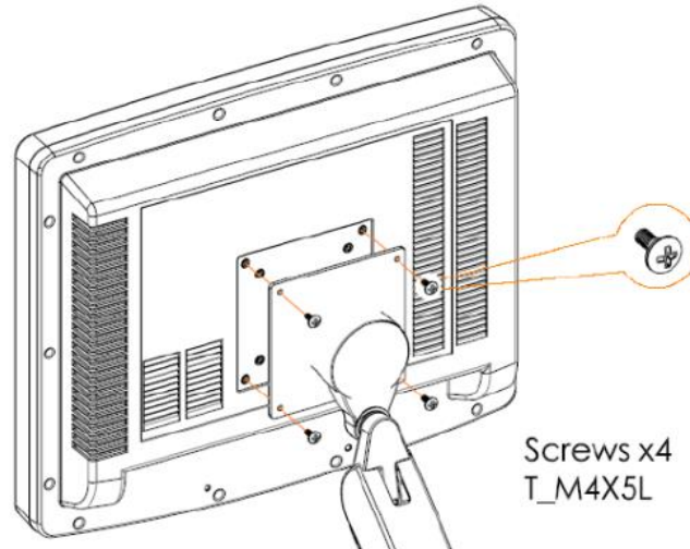
Figure 1.10: ARCHMI Series VESA Mounting
