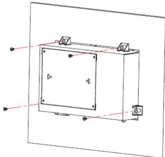
Figure 1.11: ARCHMI Series Panel Mounting
