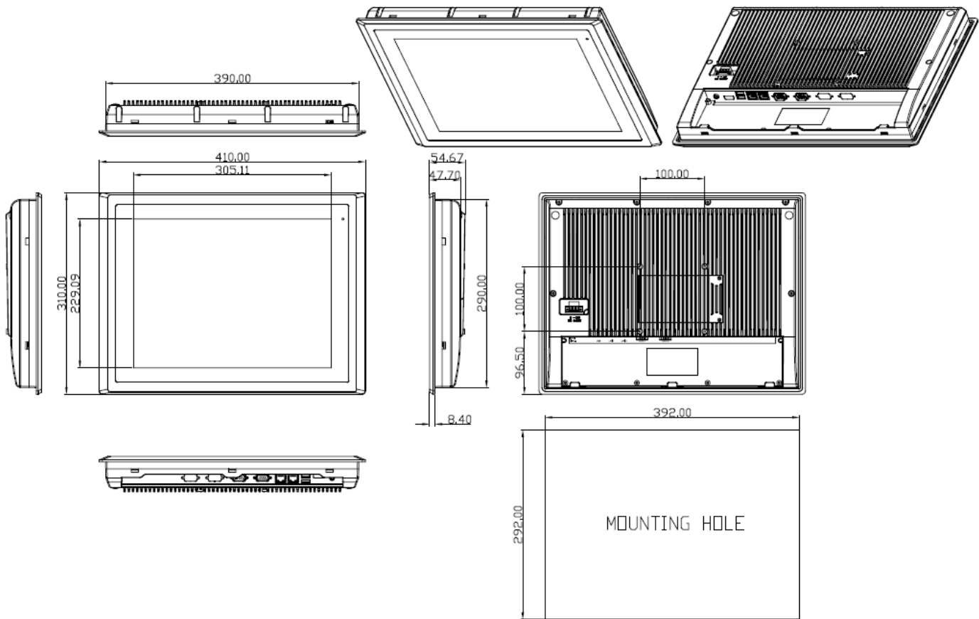
Figure 1.5: Dimensions of ARCHMI-715(P)
