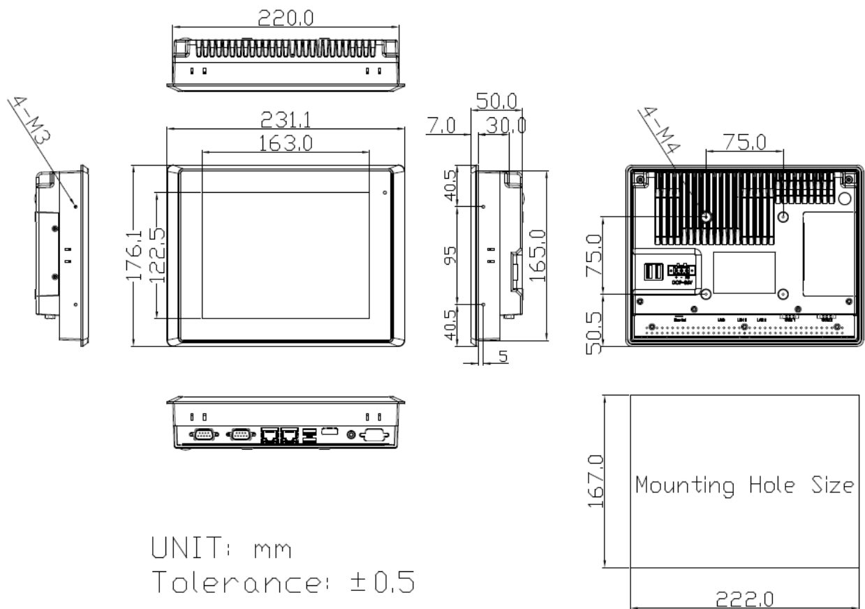
Figure 1.2: Dimensions of ARCHMI-708(P)
