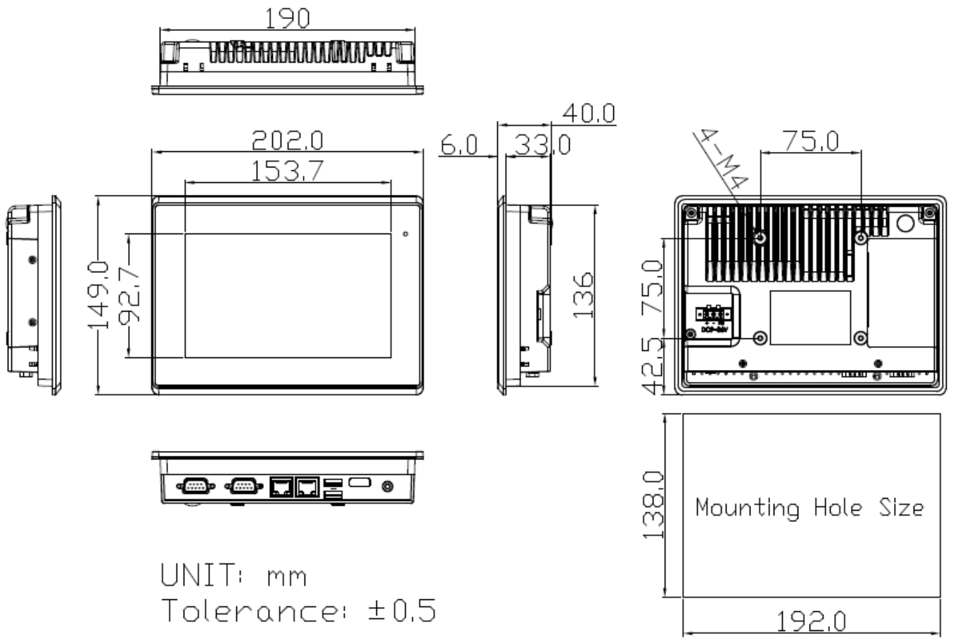
Figure 1.1: Dimensions of ARCHMI-707(P)
